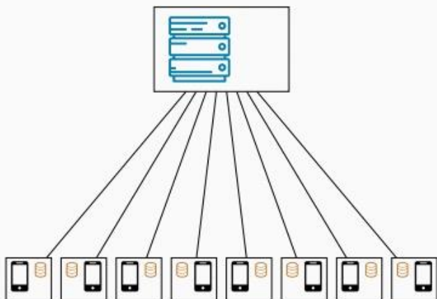
Cross-device FL
