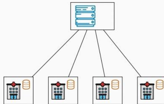
Cross-silo FL
